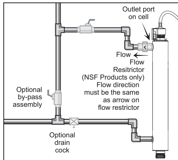
Figure 4 Flow Restrictor
